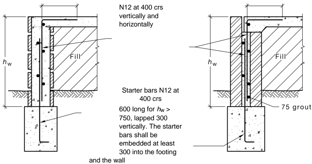
(c) Reinforced block h_w = 750 to 1500
