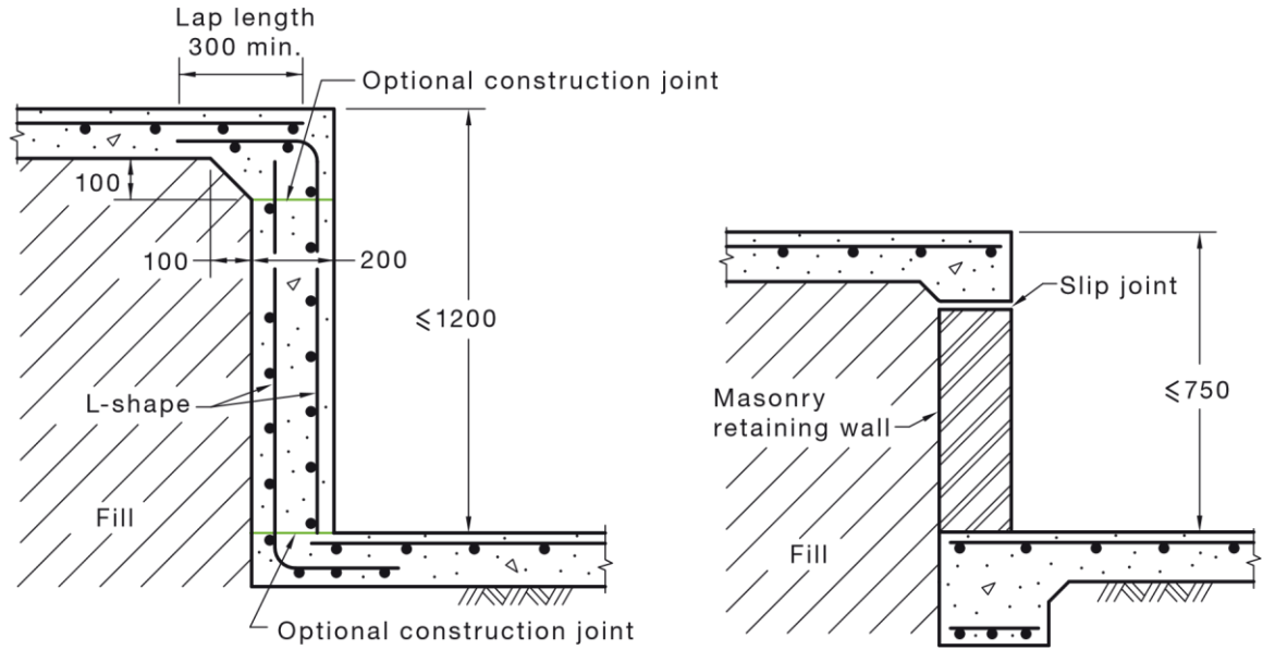
FIGURE 6.1 FILL AND SLAB EDGE OPTIONS FOR LOW SIDE OF SLOPED SITES
