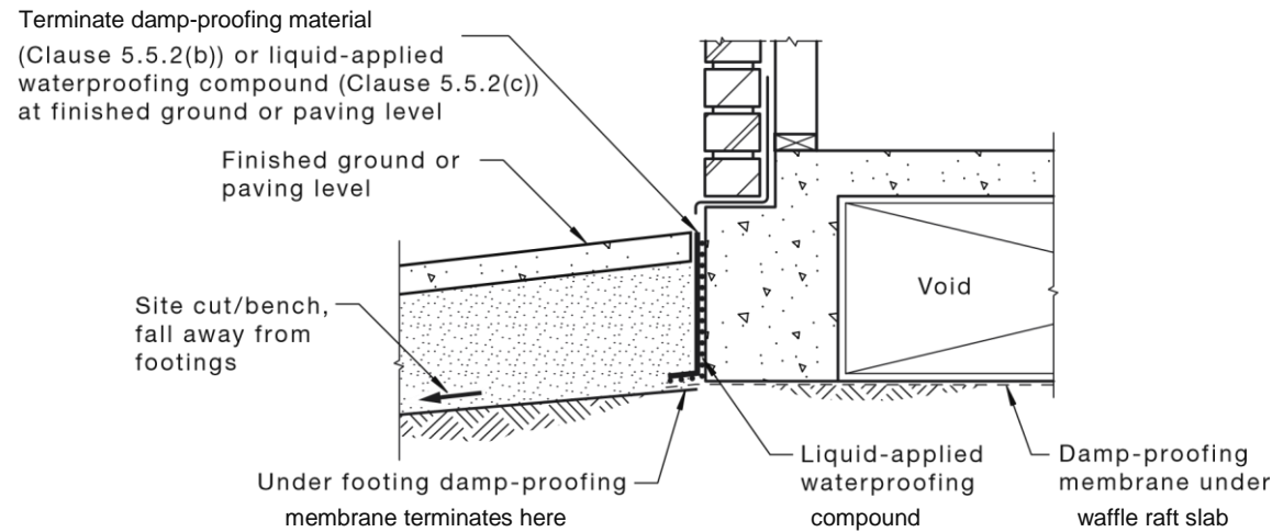
(c) Waffle raft in accordance with Clause 5.5.2(b) or 5.5.2(c)
