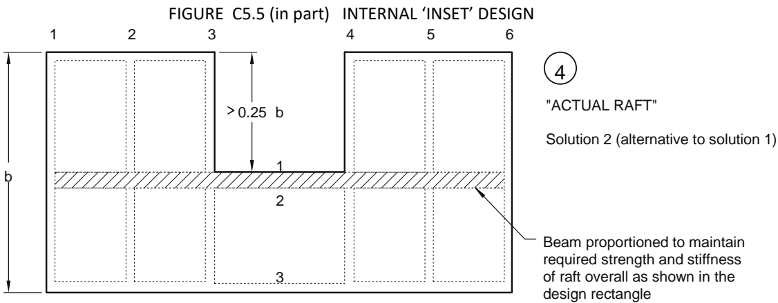
FIGURE C5.5 (in part) INTERNAL 'INSET' DESIGN
