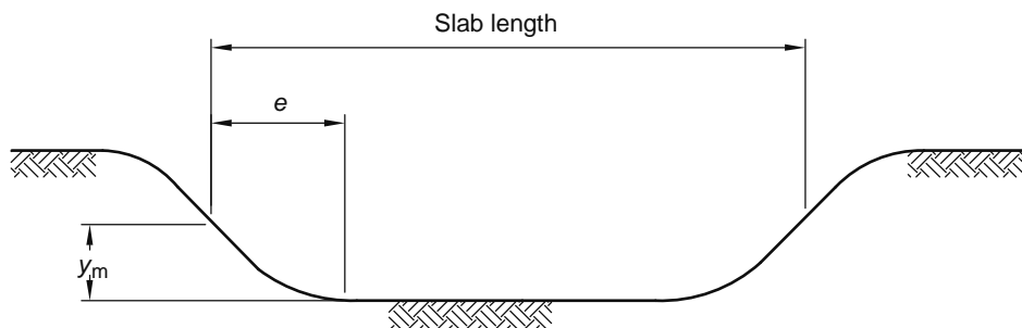
FIGURE C1 IDEALIZED GROUND MOVEMENT PATTERNS FOR FOOTINGS AND SLABS ON CLAYS (Walsh shapes)
