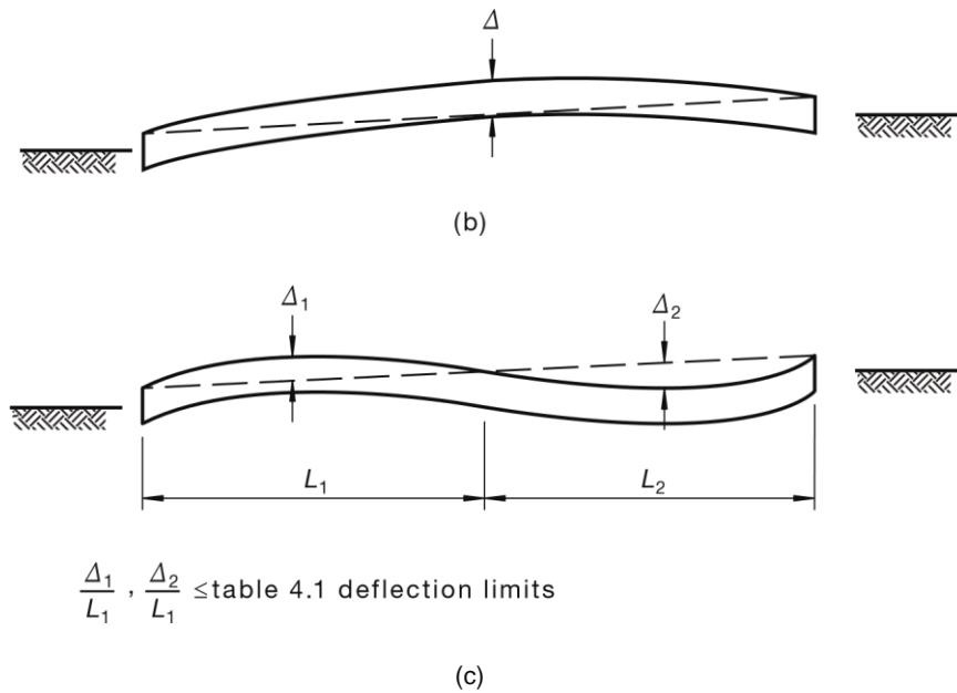
FIGURE C4.1 MEASUREMENT OF DEFLECTION
