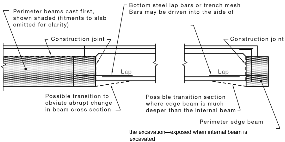
(b) Plan view of intersection of internal and edge beam
