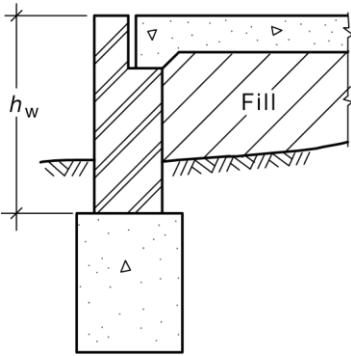
(b) Double width masonry h \leq 750
