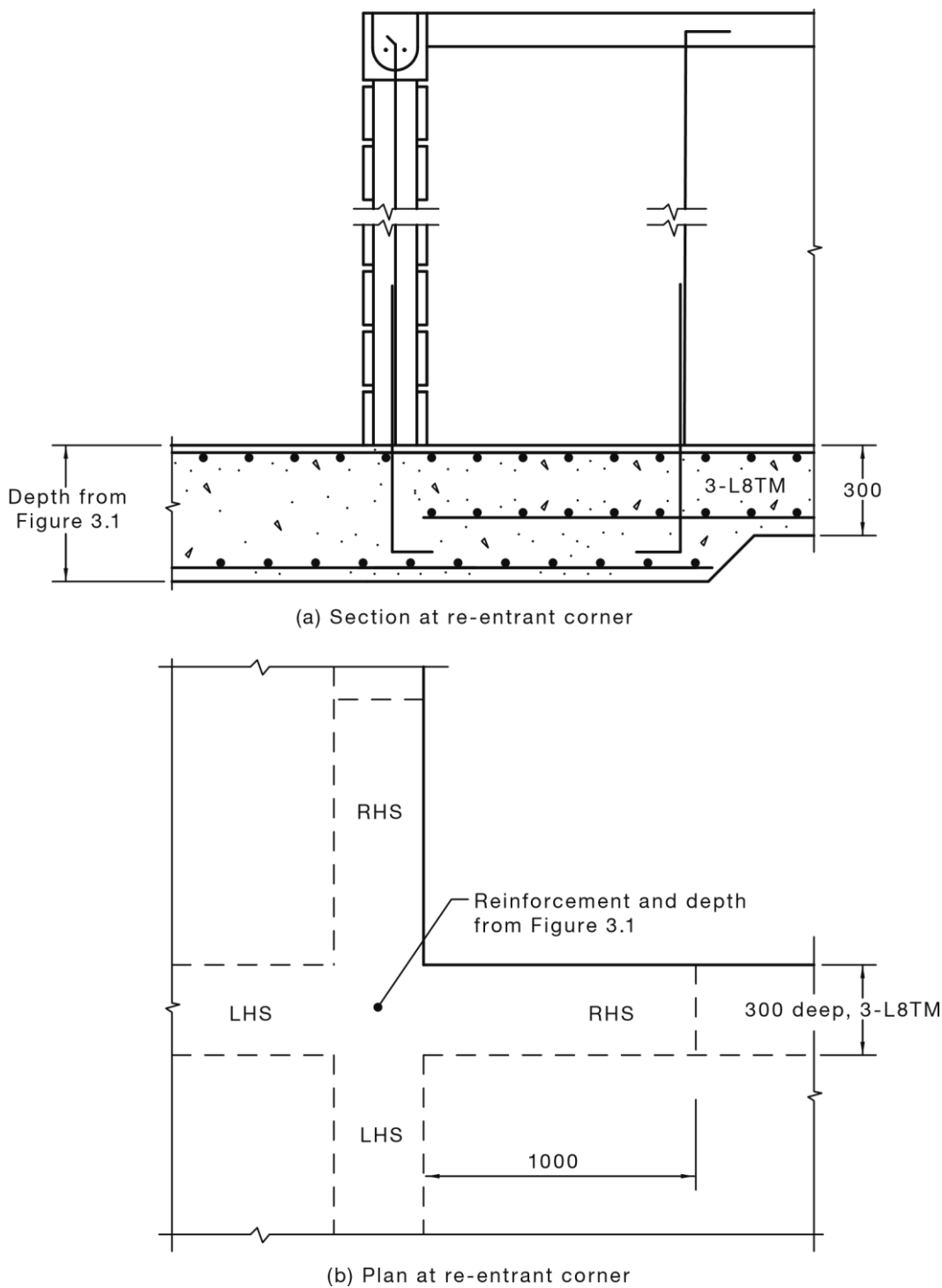
DIMENSIONS IN MILLIMETRES FIGURE C3.4 TYPICAL
