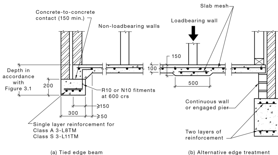
FIGURE 3.2 FOOTING SLAB FOR CLASS A SITES FOR CLAD FRAME, ARTICULATED MASONRY VENEER, MASONRY VENEER, ARTICULATED FULL MASONRY OR FULL MASONRY
