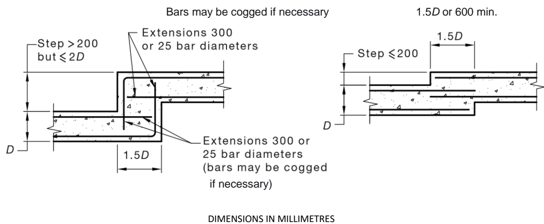
FIGURE 5.6 ACCEPTABLE METHODS OF STEPPING STRIP FOOTINGS
