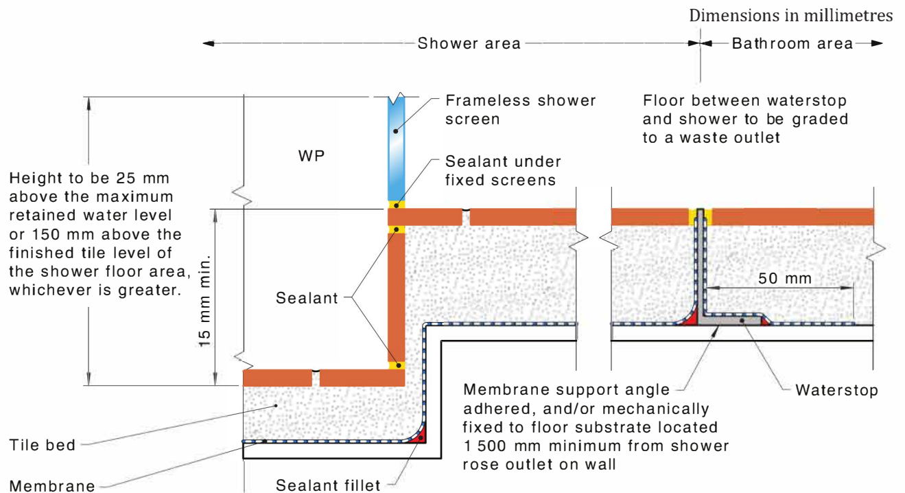
Figure 4.8.2(A) — Unenclosed shower — Membrane below tile bed
